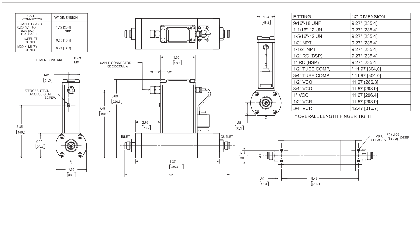
Figure 4 Model SLAMf53 with Cable Gland (PG11, M20 x 1.5, 1/2" NPT) MFC (See Instruction Manual for SLAMf53 with Flanged Connections Details)
