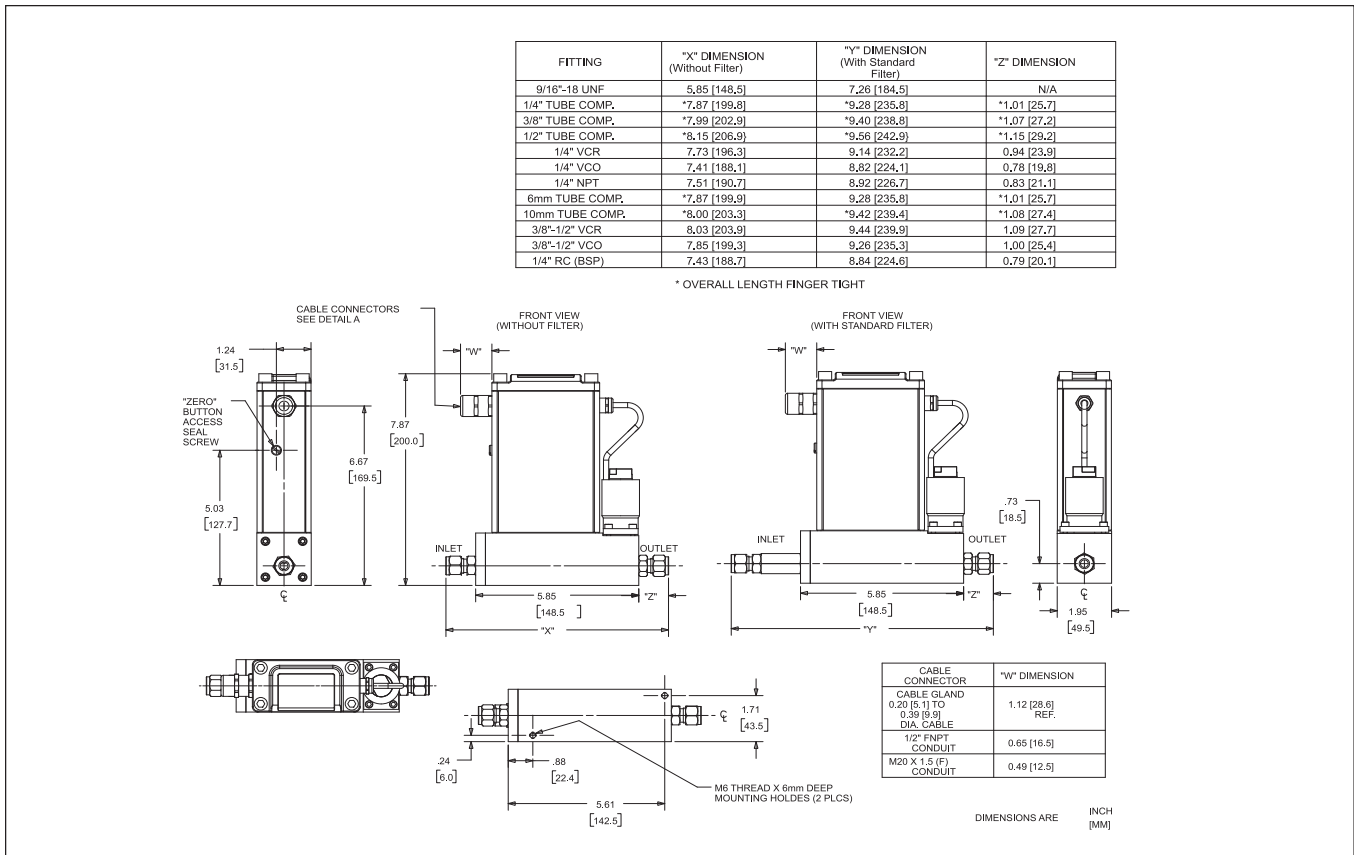
Figure 3 Model SLAMf51 with Cable Gland (PG11, M20 x 1.5, 1/2" NPT) MFC
