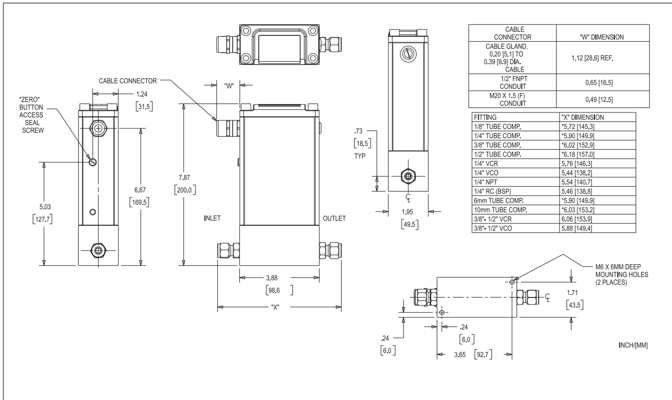
6 Figure 6 Model SLAMf60 with Cable Gland (PG11, M20 x 1.5, 1/2" NPT) MFM
