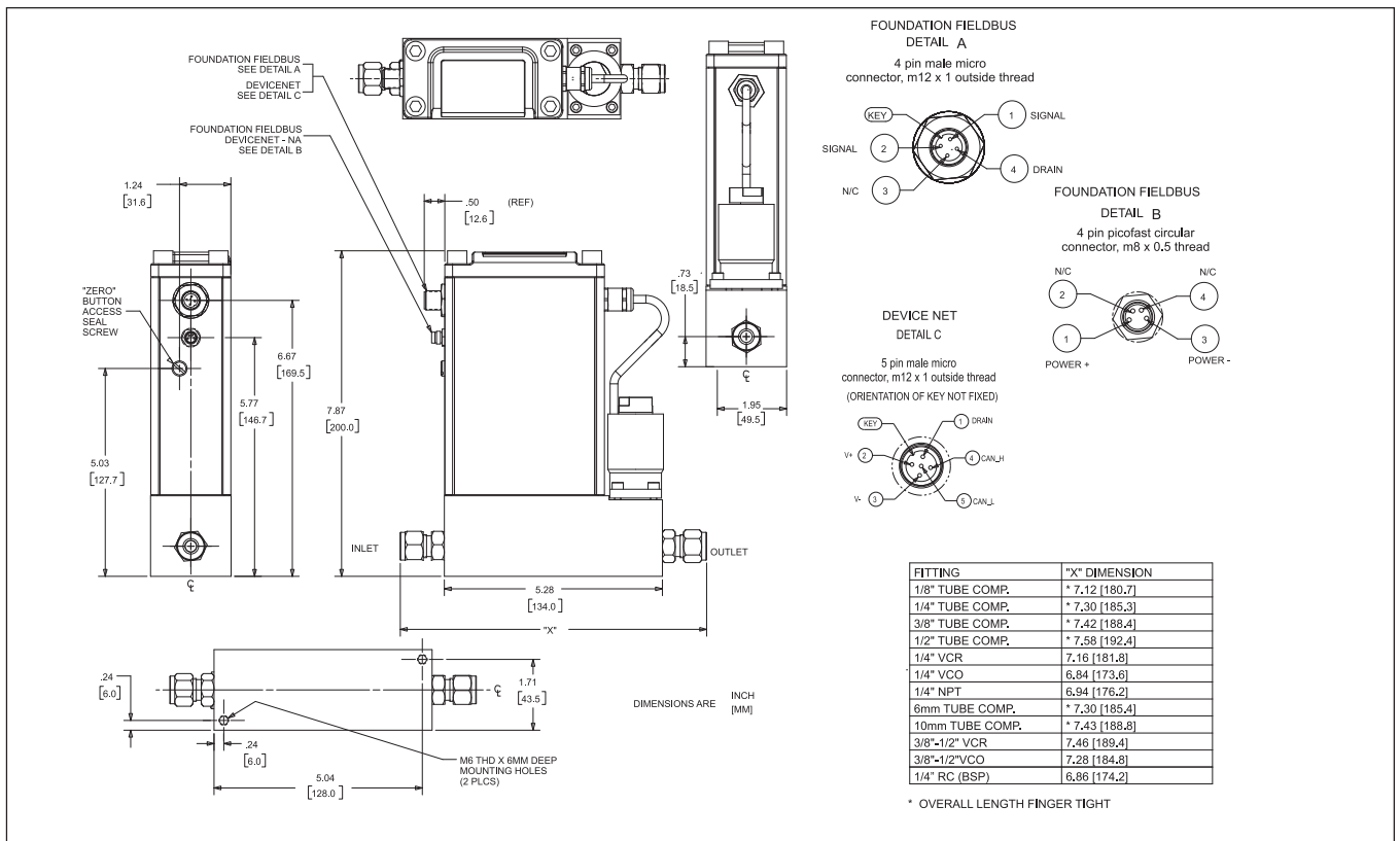
Figure 2 Model SLAMf50D Digital I/O DeviceNet MFC and Model SLAMf50F Digital I/O Foundation Fieldbus
