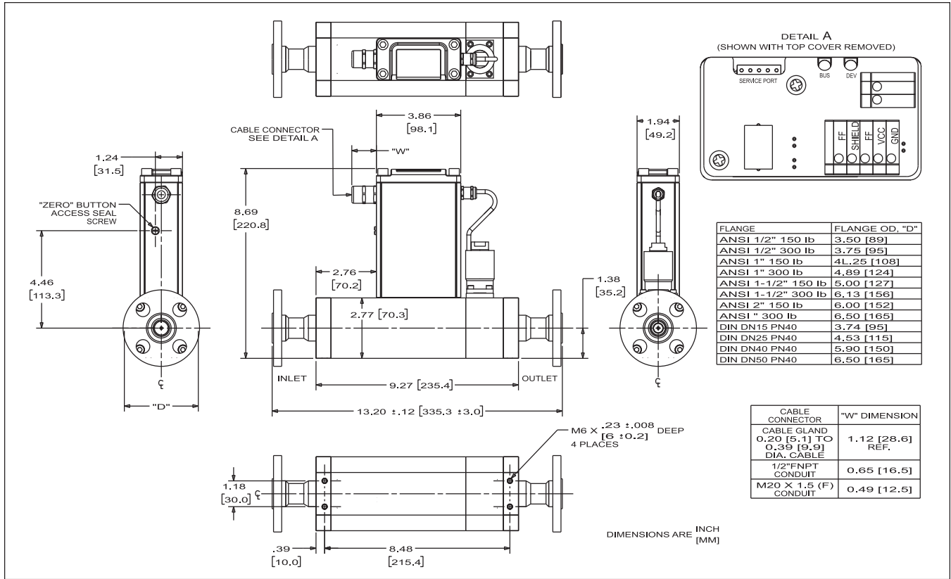
Figure 5 Model SLAMf53 with Cable Gland (PG11, M20 x 1.5, 1/2" NPT) with Flanged Connections MFC
